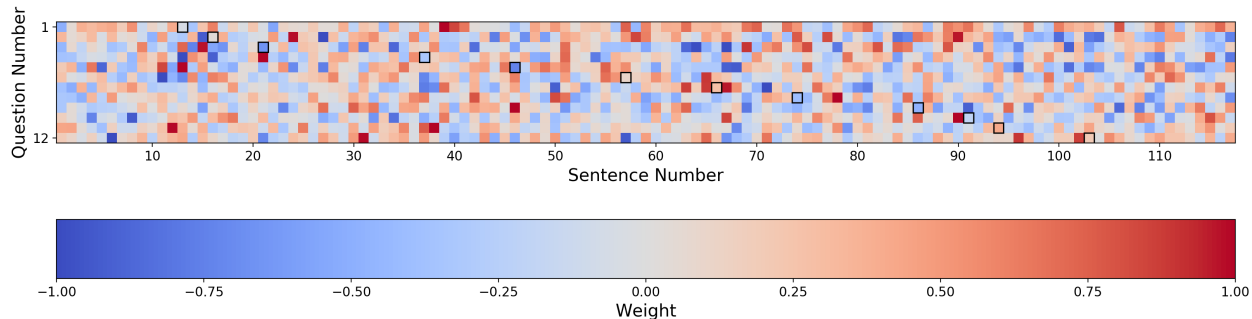
Figure 4: Mean highlighting weights, \omega_{c_i} , for models trained on the sentence representation. The weights are normalized by question such that the magnitude of the largest weight is 1.0. The black squares indicate which highlight features were used to generate each quiz question.
