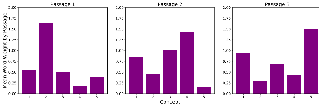
Figure 8: Bar graphs of the mean word weighting in the given concept for each of the three passages taken from one fold of the cross validation.
